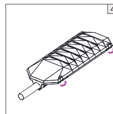
4. Fixate it with the screws and connect the cable back. Close and lock the cover. LED module maintenance finished.
