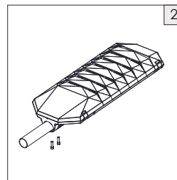
2. Connect the wires to AC input. Insert the arm/post into the sleeve, and tighten up the two screws. Installation finished.
