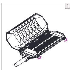
1. Undo the three buckles to open the cover.
