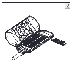
2. Undo the two screws on the ends of the failed LED module, disconnect the cable connector, and take out the module.
